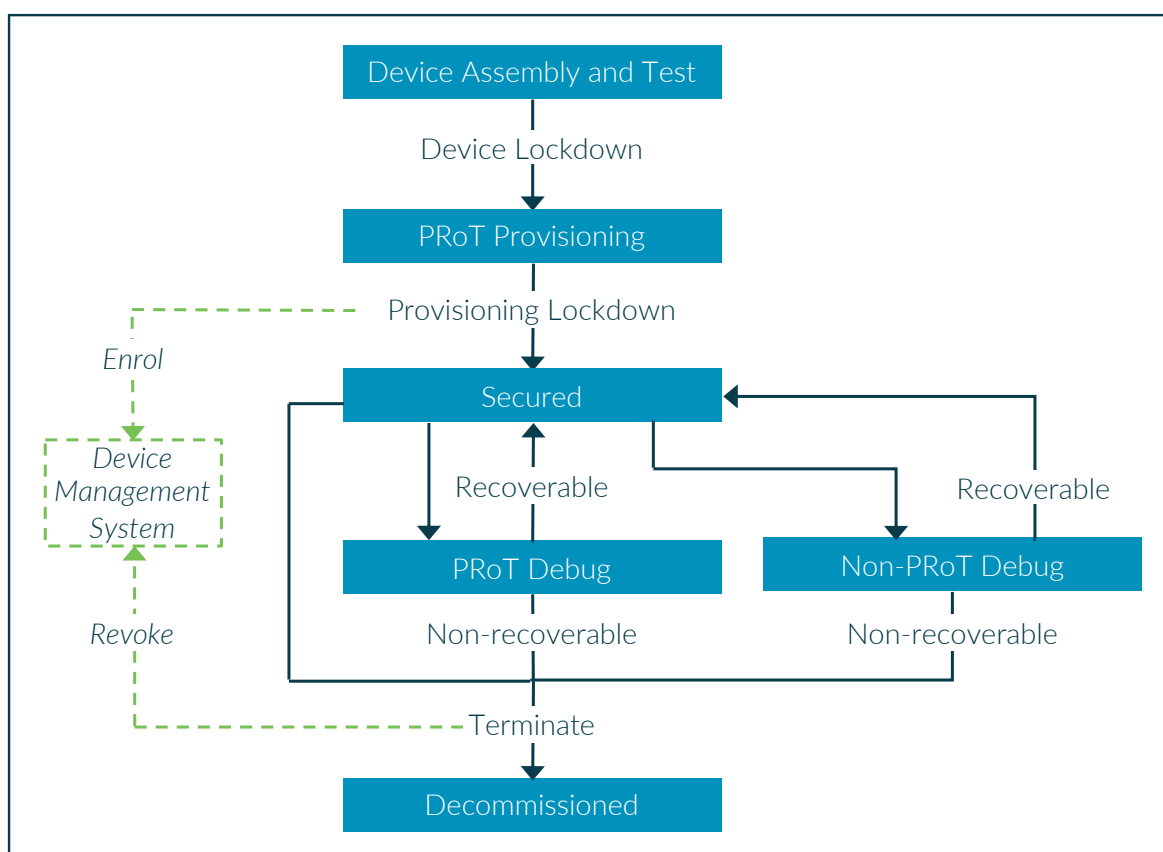
Figure 11 : Generic Platform Root of Trust security lifecycle
