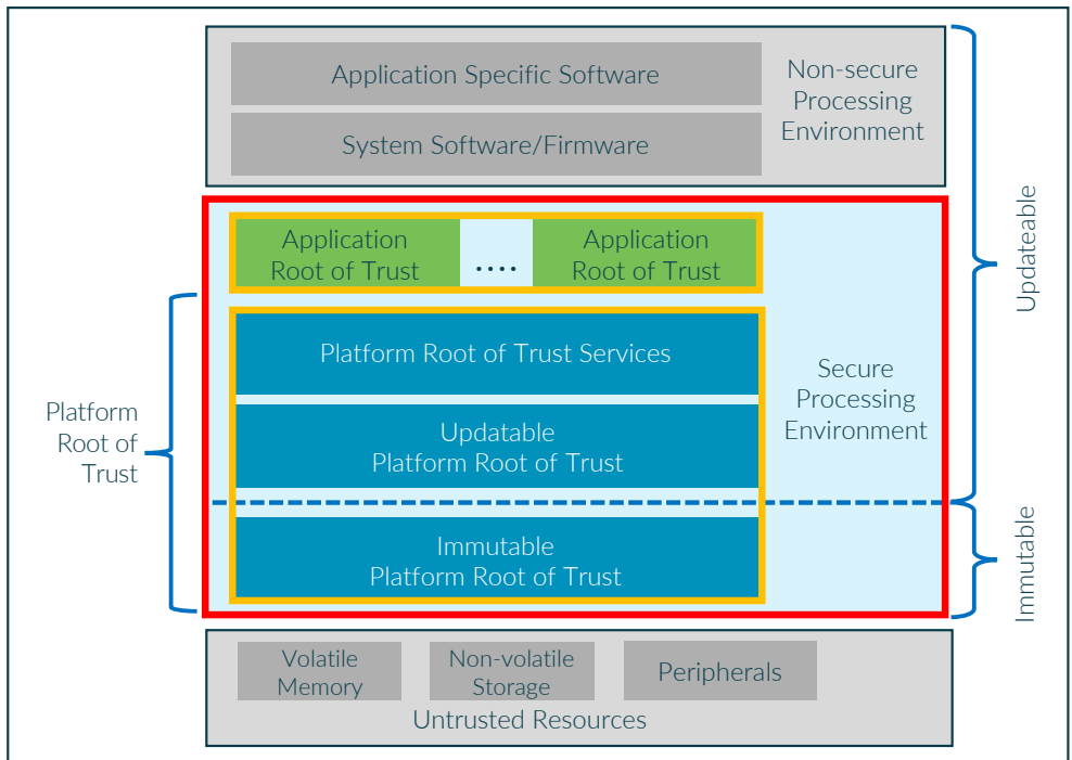
Figure 6: ARoT/PRoT secure partition isolation
