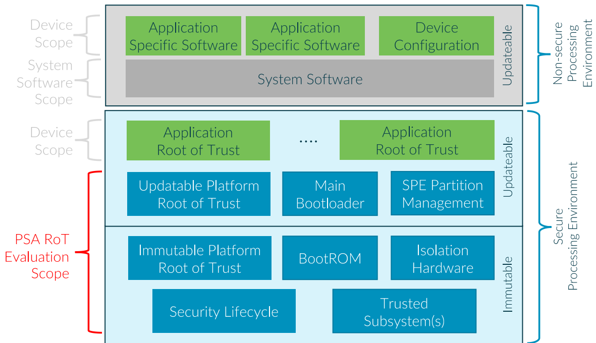
Figure 1: Scope of PSA Certified Level 3
